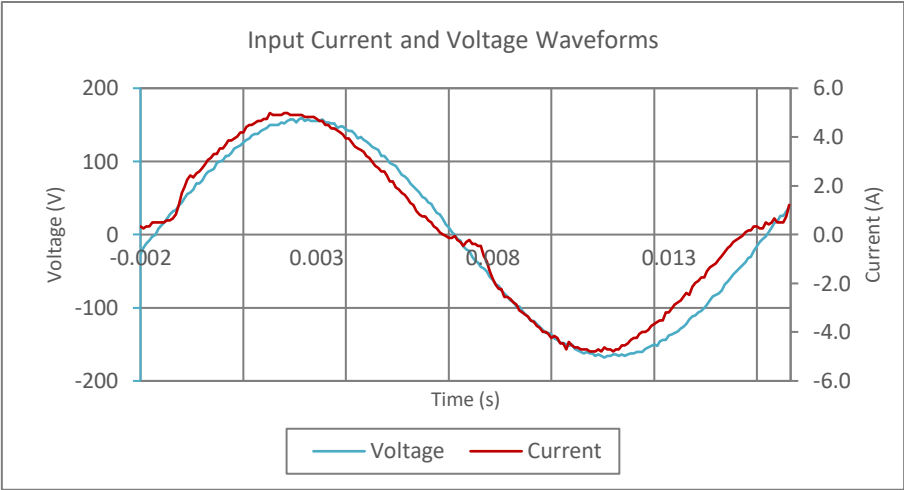
Input AC Current Waveform (ITHD = 9.64%, 50% Load)
